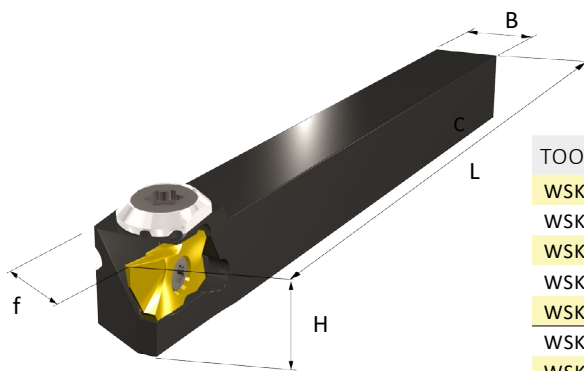
WhizFix Clamping
