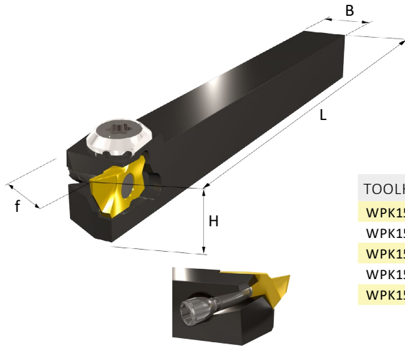
WhizFix Clamping
